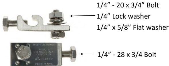
WEEB Grounding Lug
